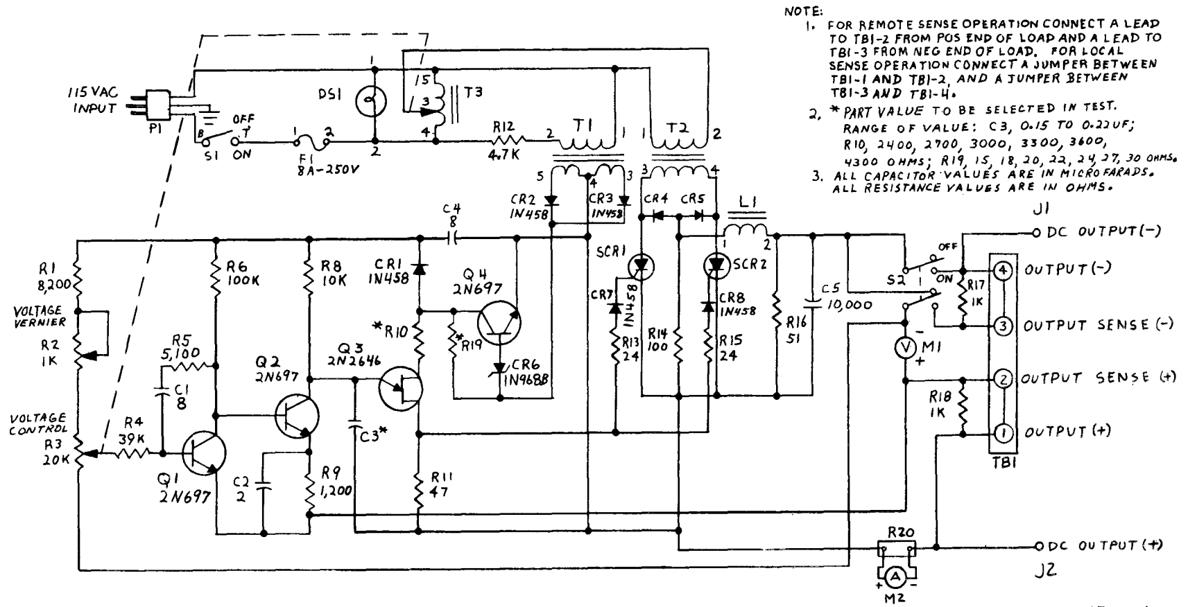
Figure 6-1. Power Supply PP-2309A/U, schematic diagram.
